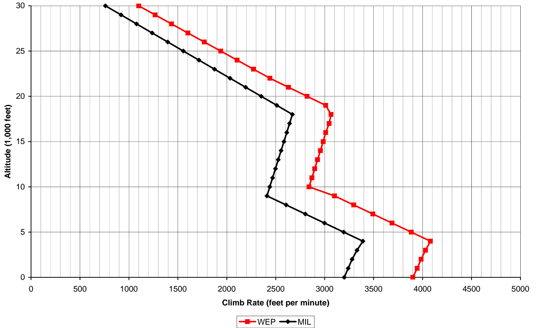
Aces High II Fw 190A-5 Climb Rate
