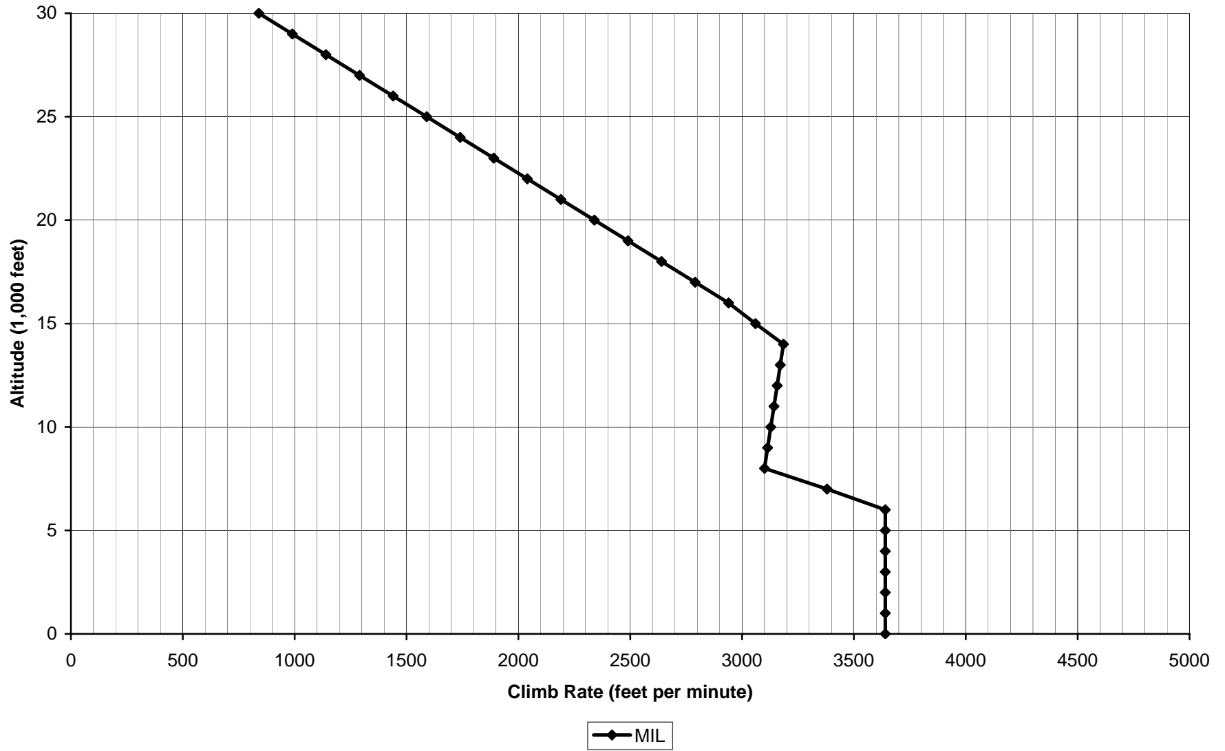
Aces High II Yak-9U Climb Rate
