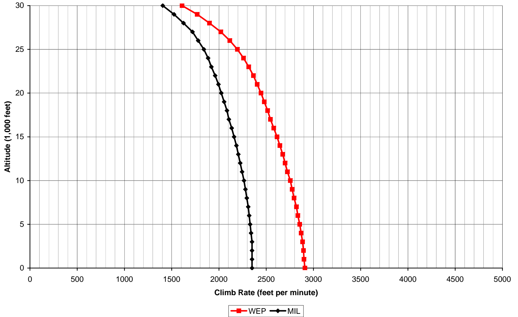
Aces High II P-47D-11 Climb Rate
