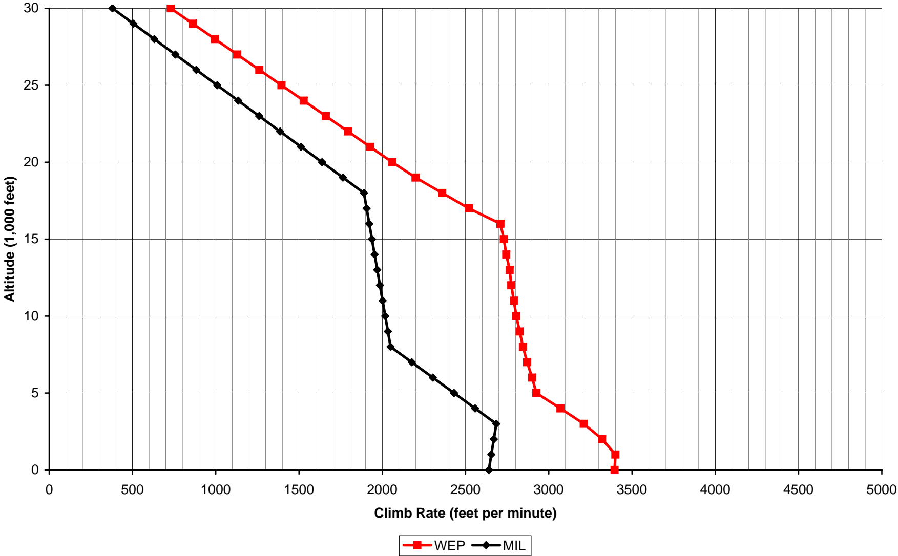
Aces High II Fw 190A-8 Climb Rate
