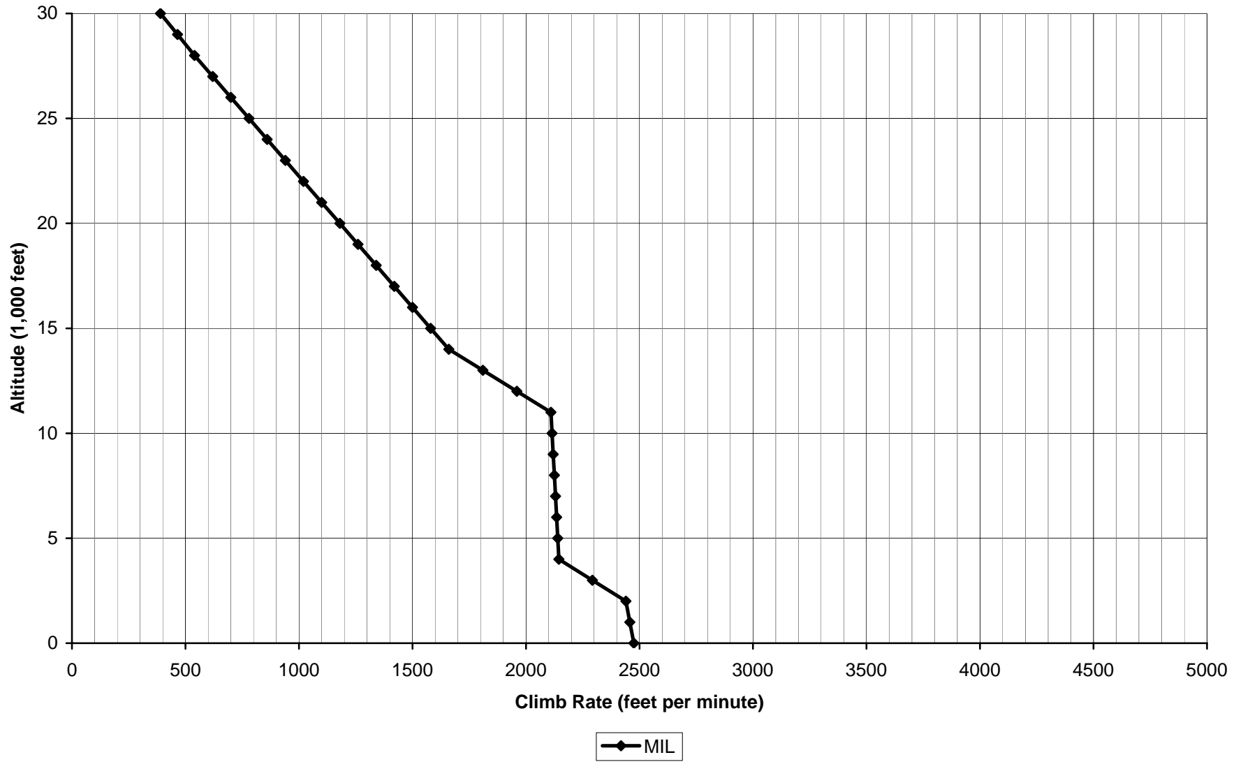
Aces High II F4F-4 Climb Rate
