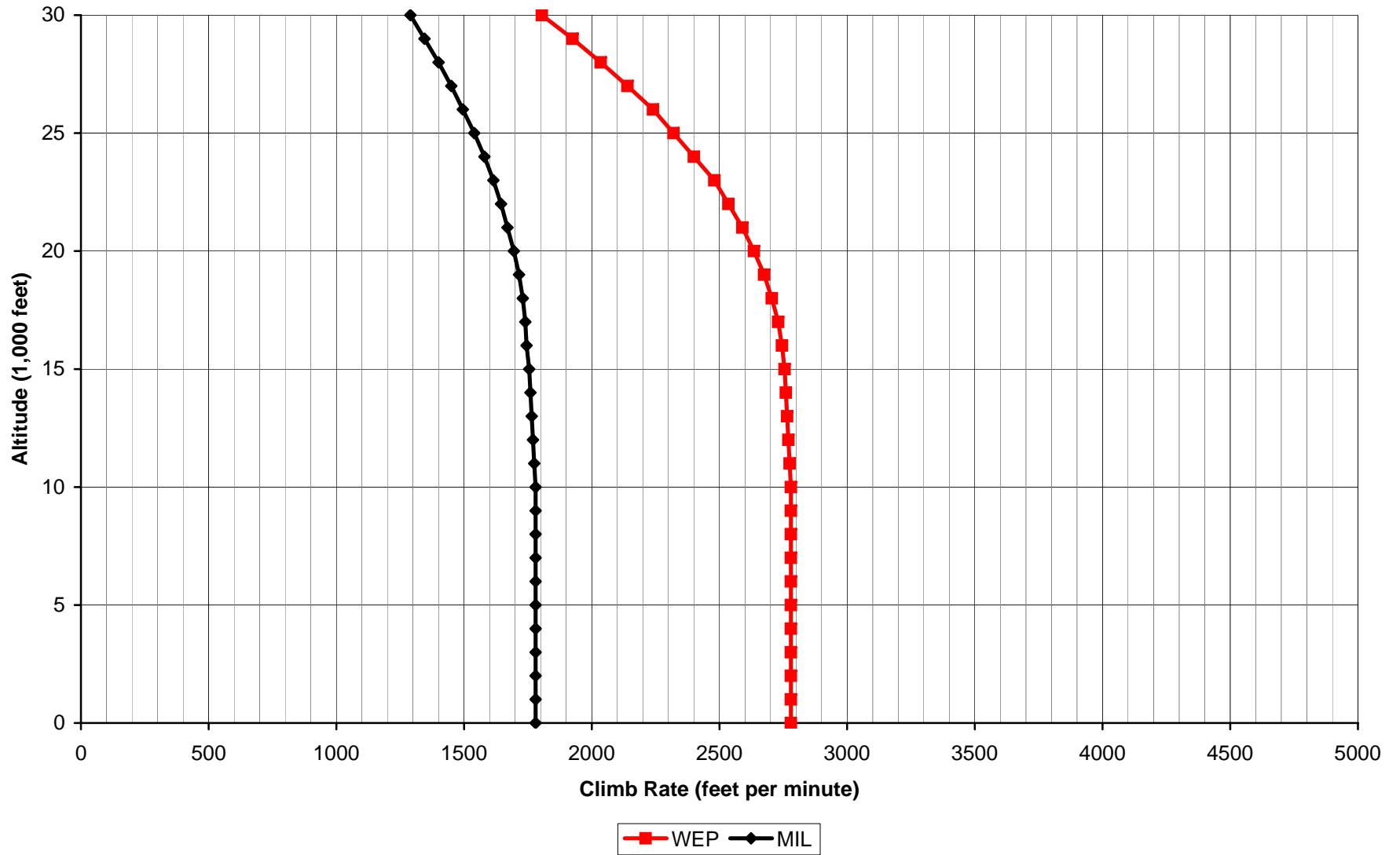
Aces High II P-47N Climb Rate
