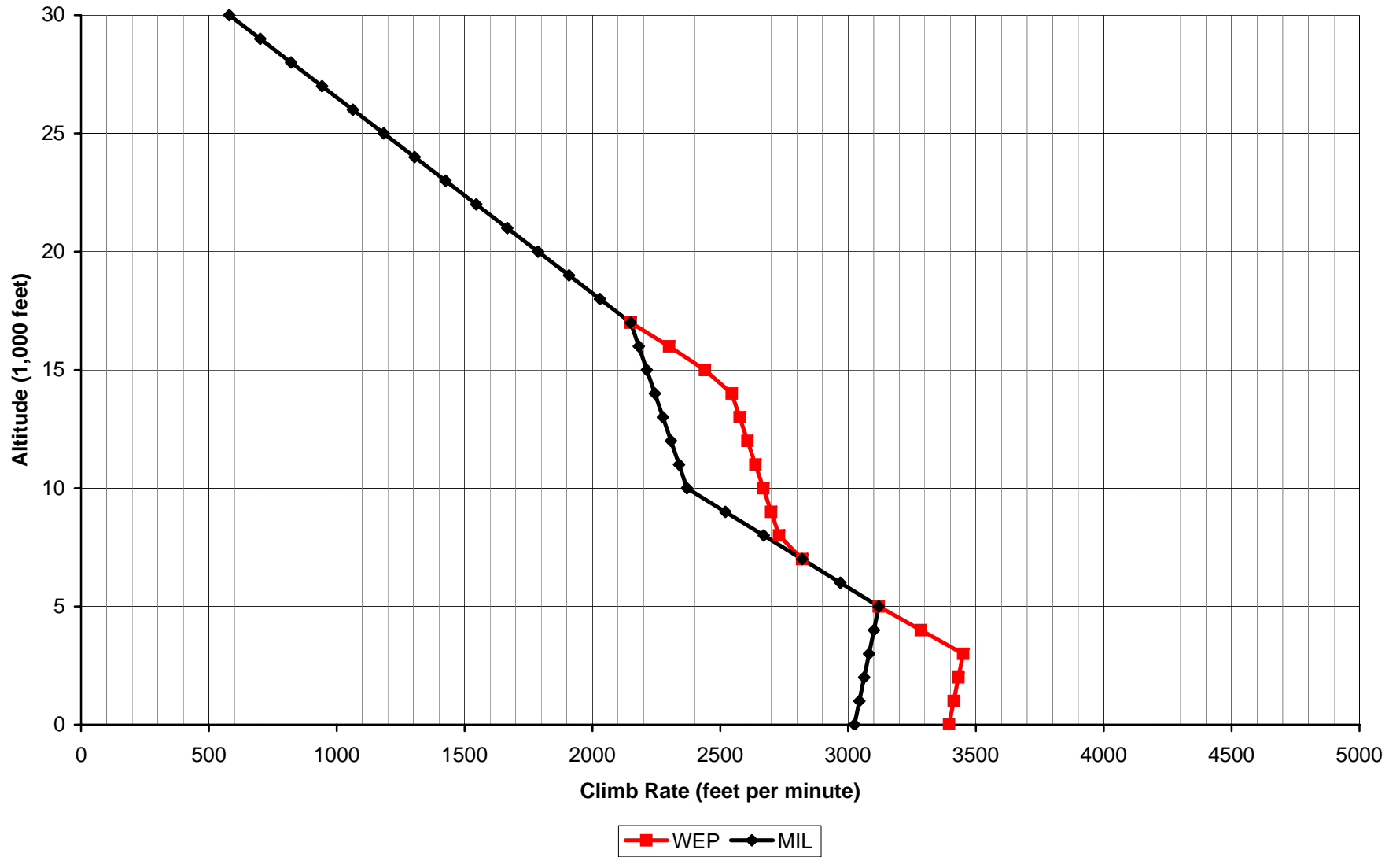
Aces High II Typhoon Climb Rate
