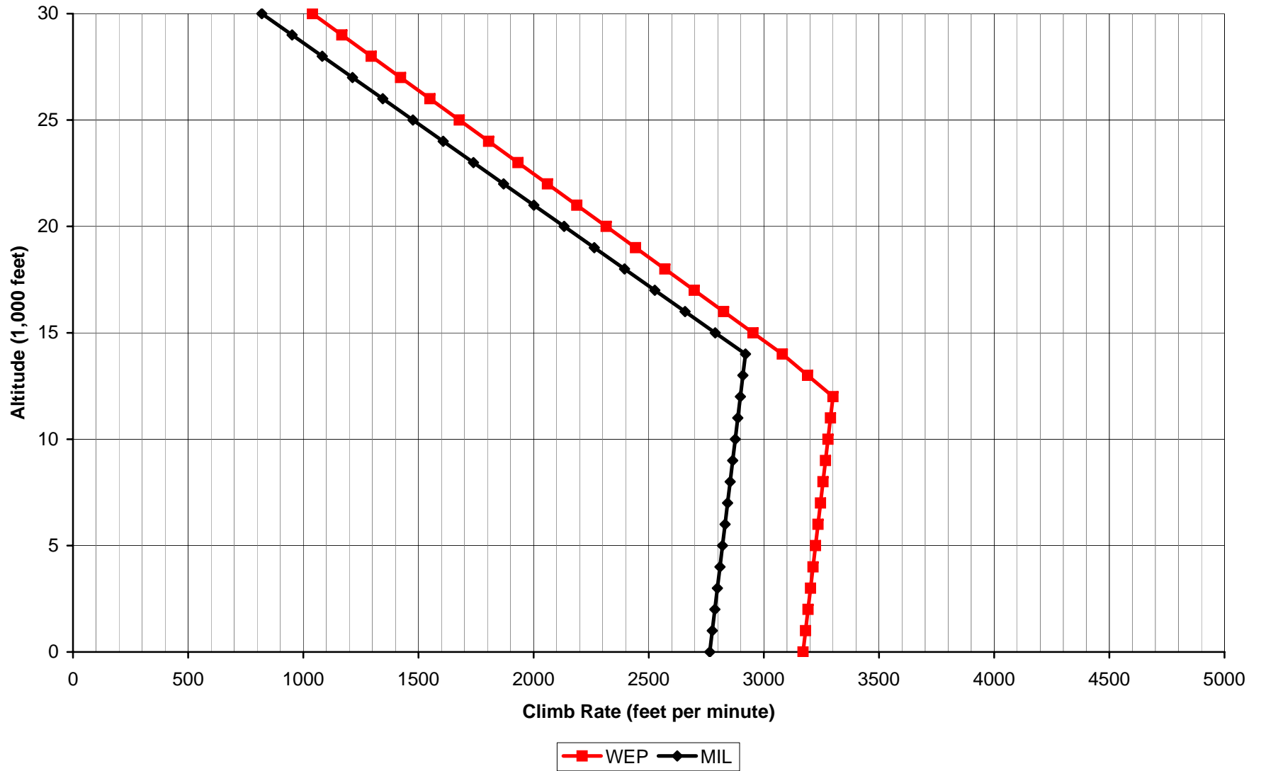
Aces High II Spitfire Mk V Climb Rate
