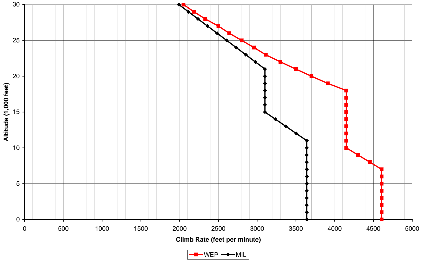
Aces High II Spitfire Mk VIII Climb Rate
