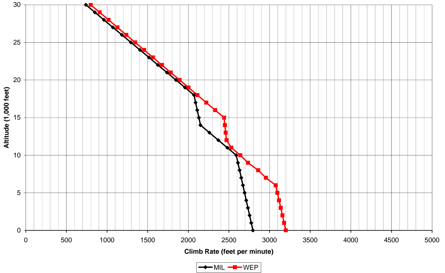
Aces High II Hurricane Mk IIC Climb Rate
