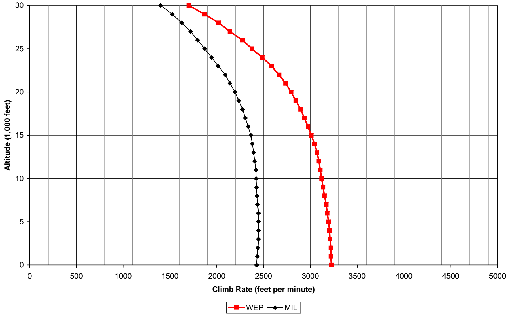
Aces High II P-47D-40 Climb Rate
