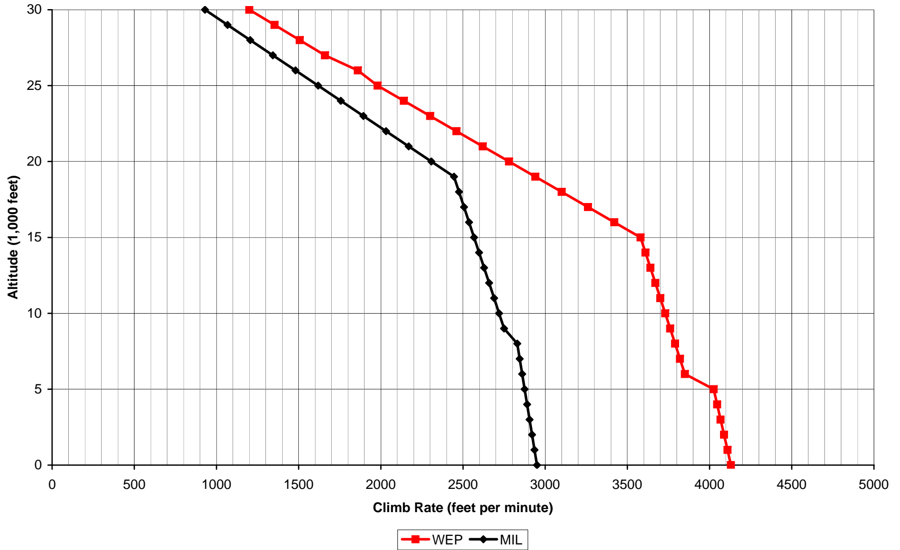
Aces High II Fw 190D-9 Climb Rate
