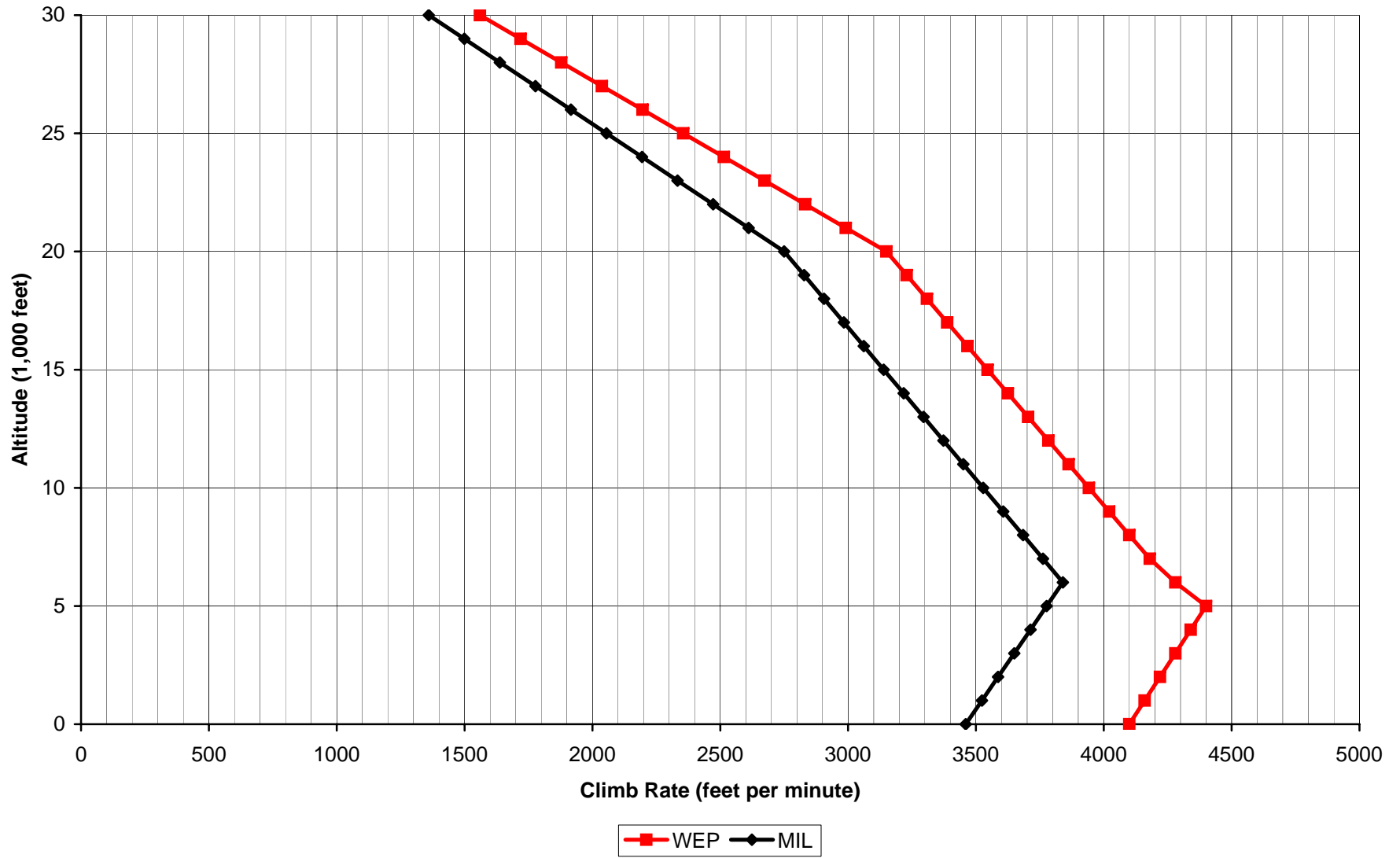
Aces High II Bf 109G-2 Climb Rate
