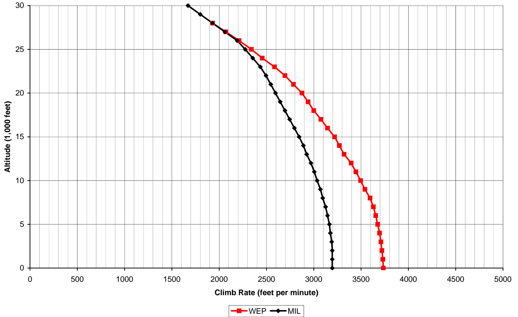
Aces High II P-38L Climb Rate
