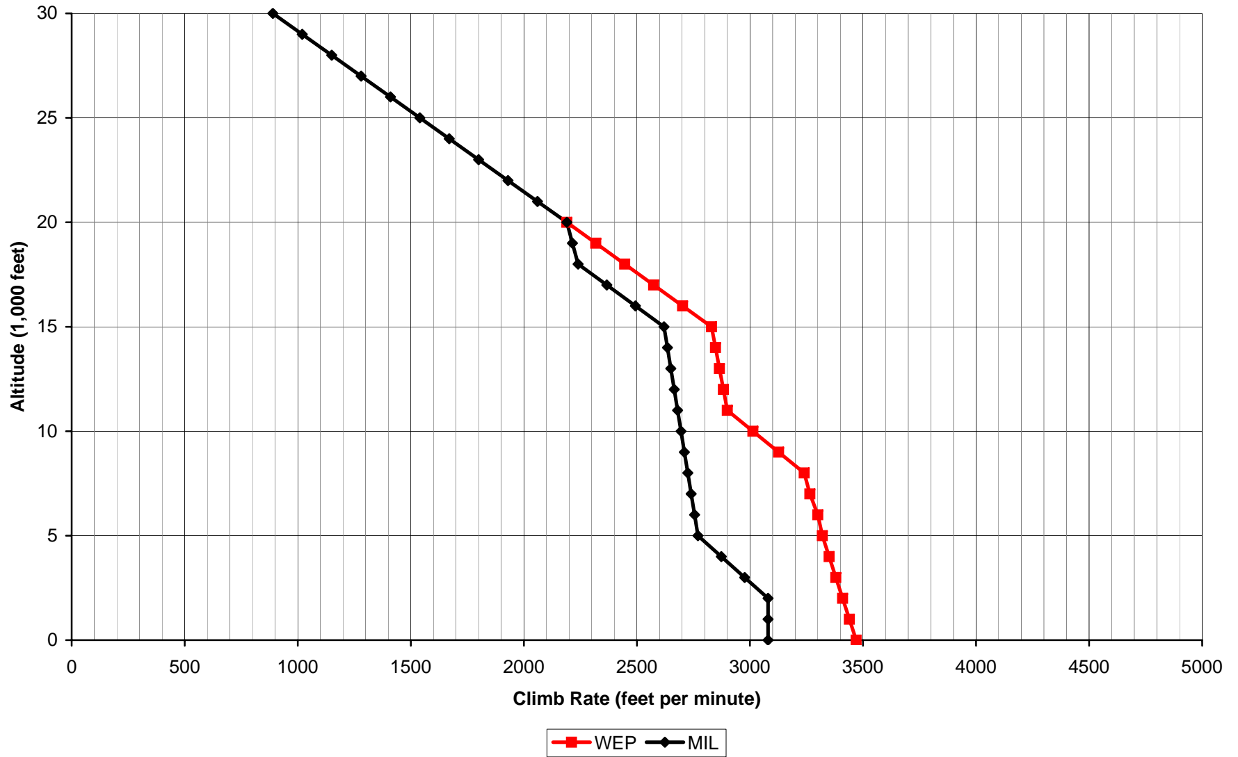
Aces High II F6F-5 Climb Rate
