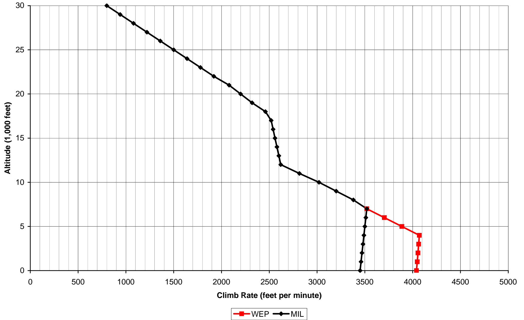
Aces High II N1K2-J Climb Rate
