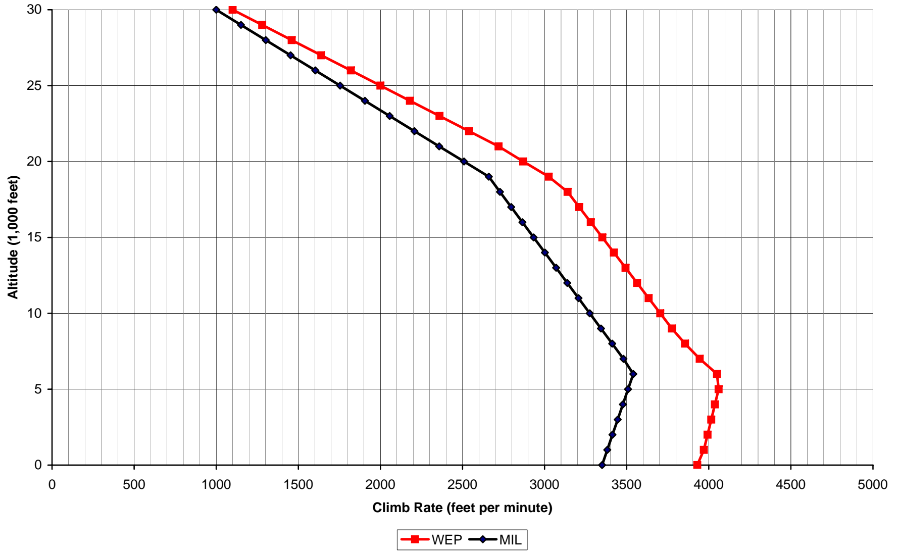
Aces High II C.205 Climb Rate
