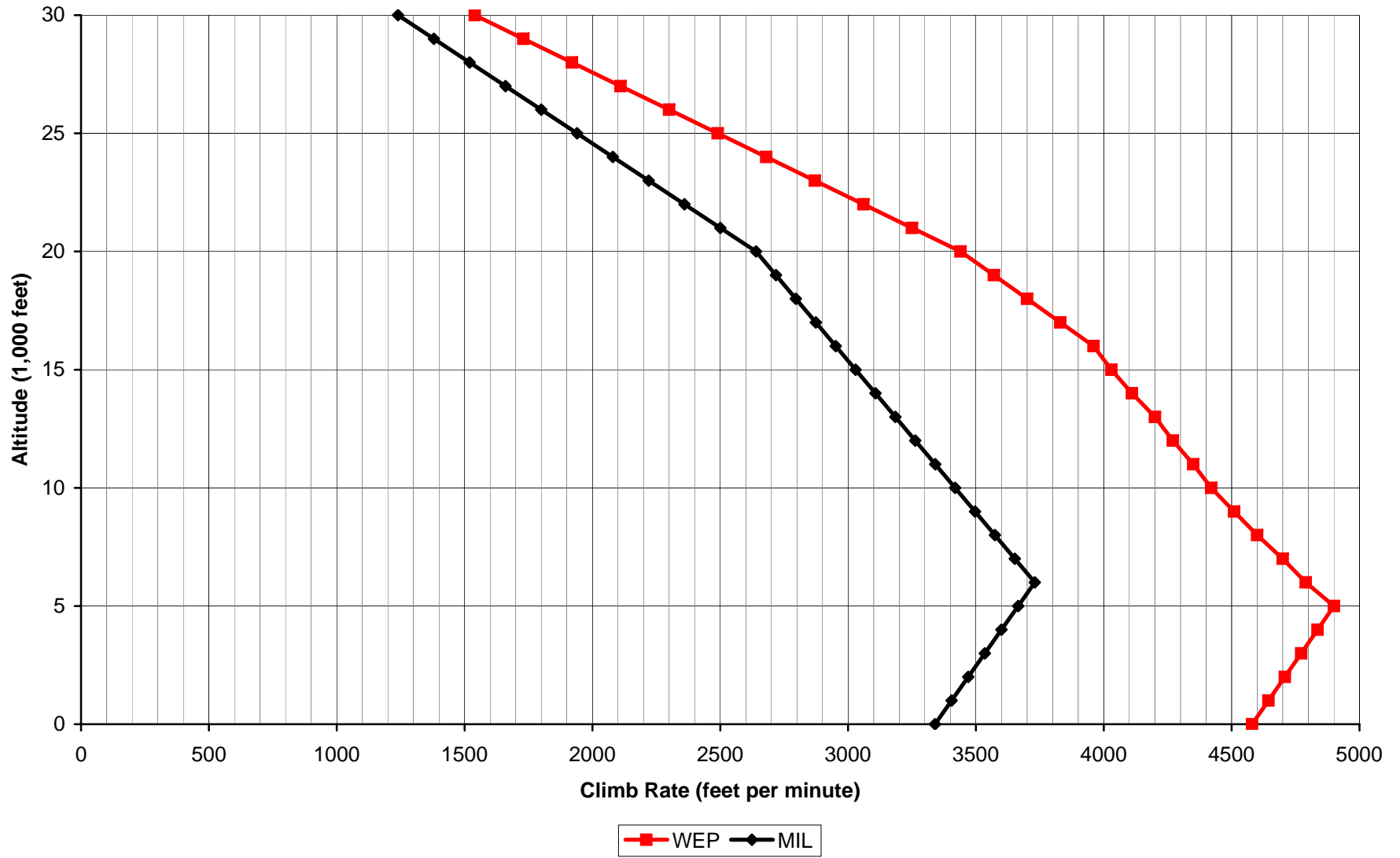
Aces High II Bf 109G-14 Climb Rate
