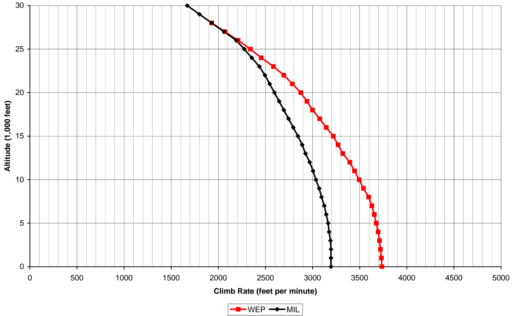
Aces High II P-38J Climb Rate
