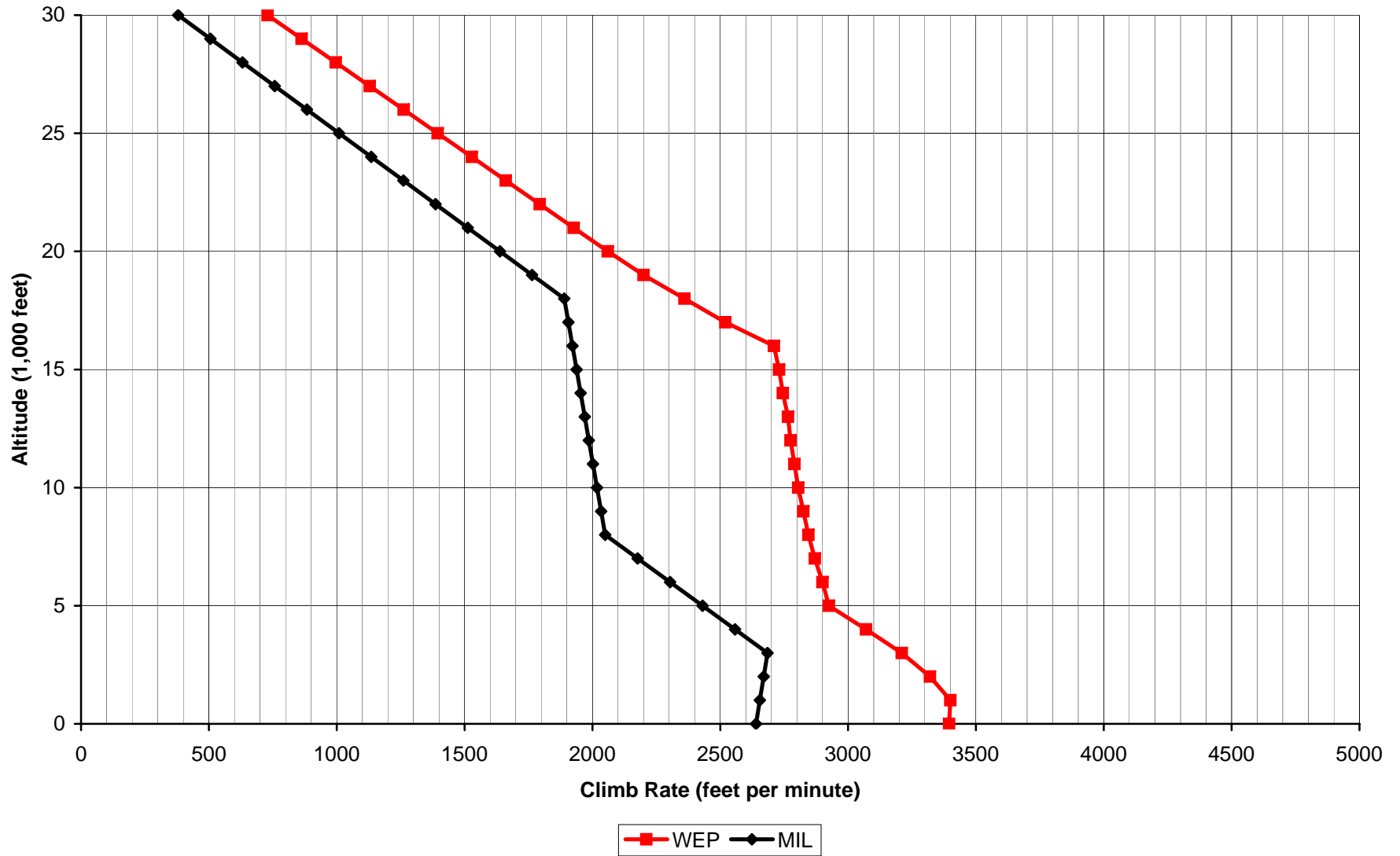
Aces High II Fw 190F-8 Climb Rate
