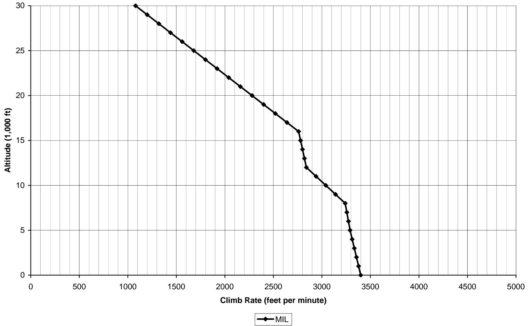
Aces High II A6M5b Climb Rate
