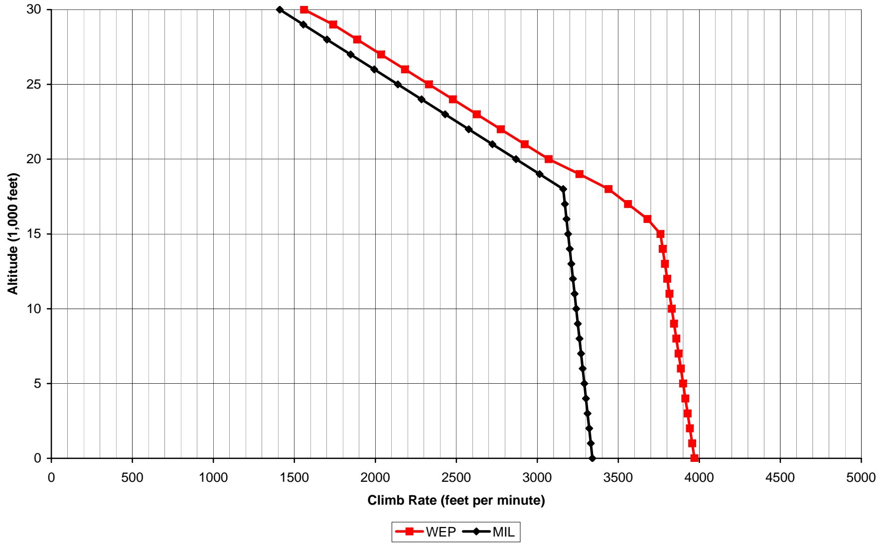
Aces High II Bf 109F-4 Climb Rate
