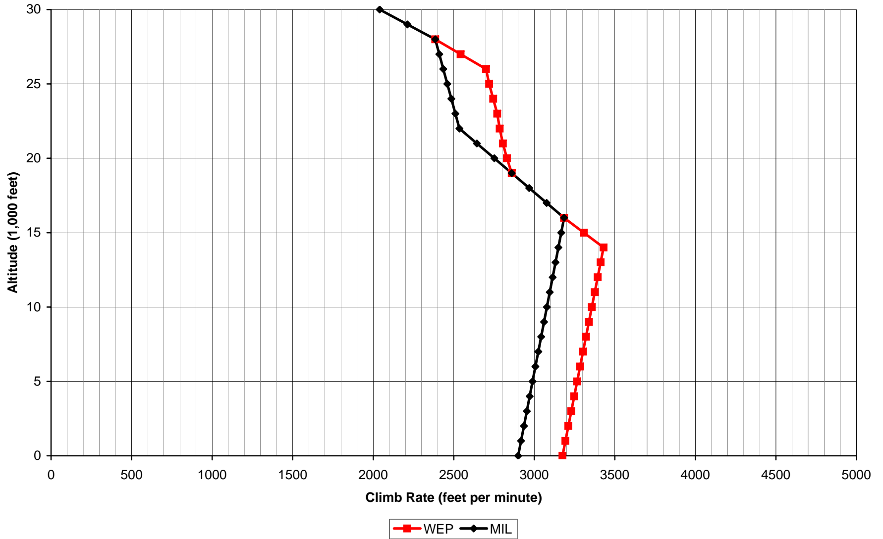
Aces High II P-51B Climb Rate
