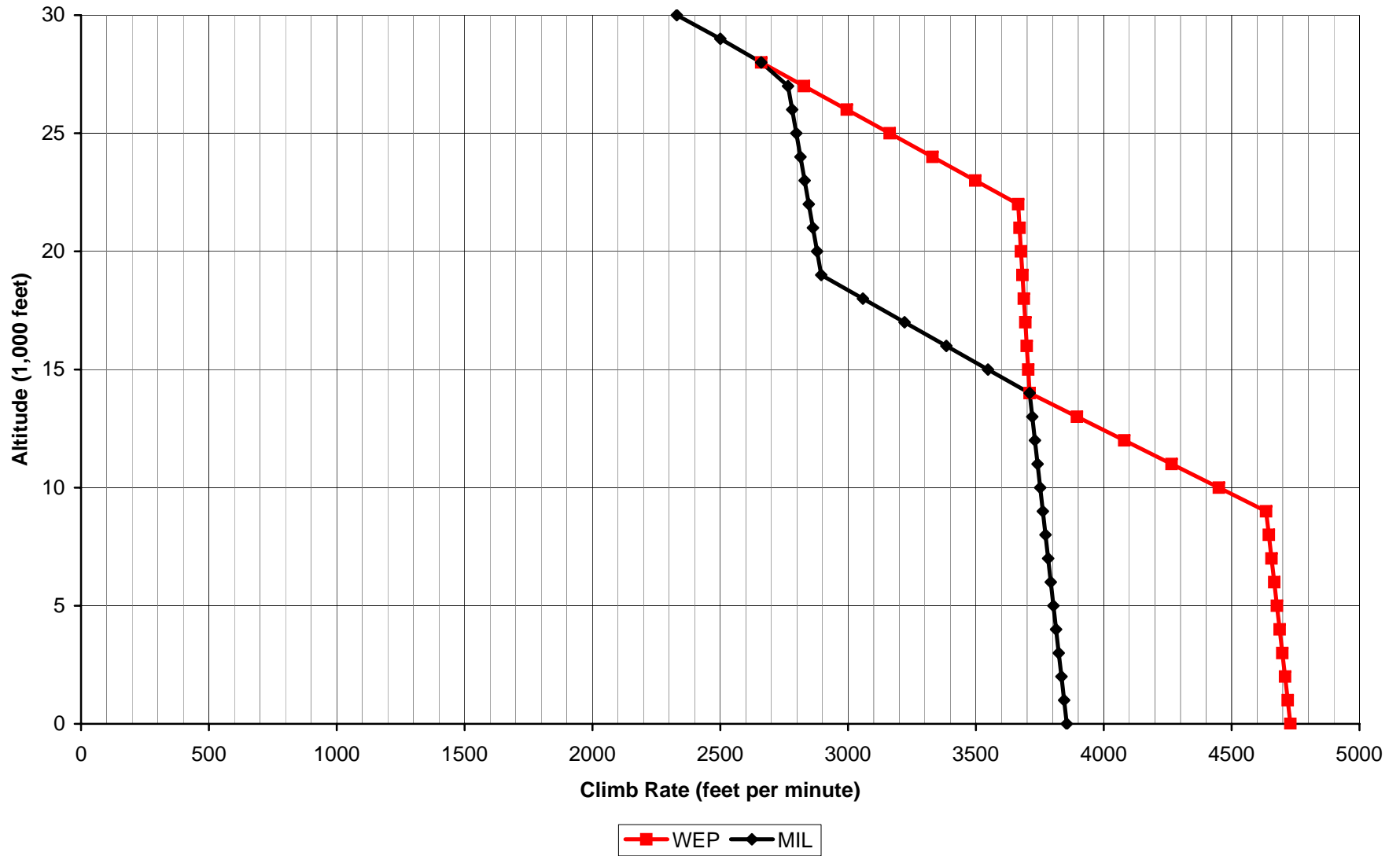
Aces High II Spitfire Mk XIV Climb Rate
