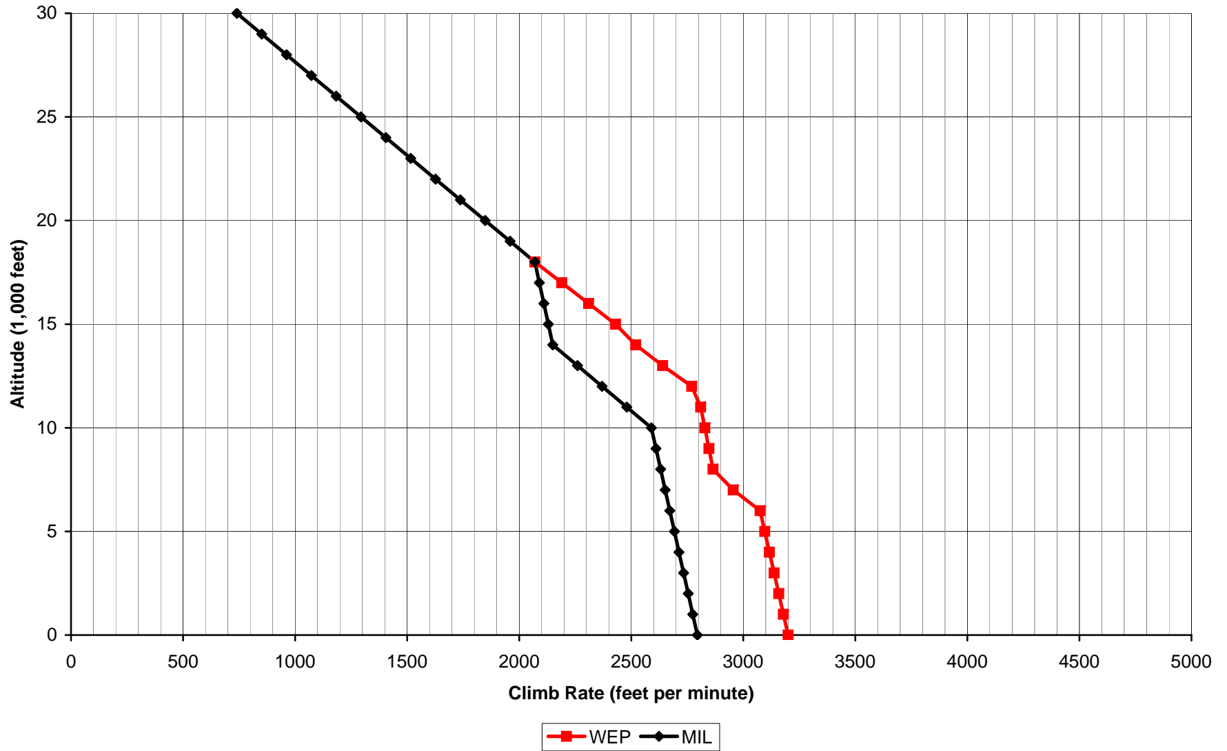
Aces High II Hurricane Mk IID Climb Rate
