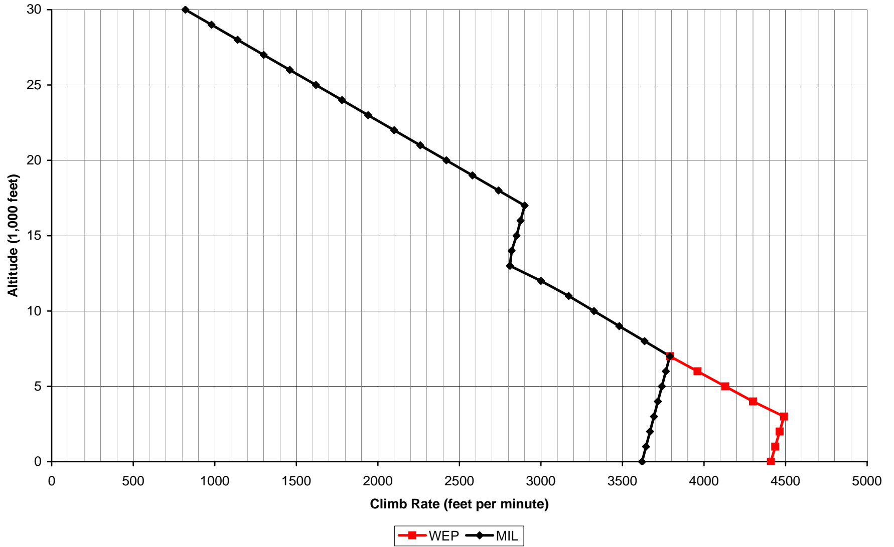
Aces High II La-7 Climb Rate
