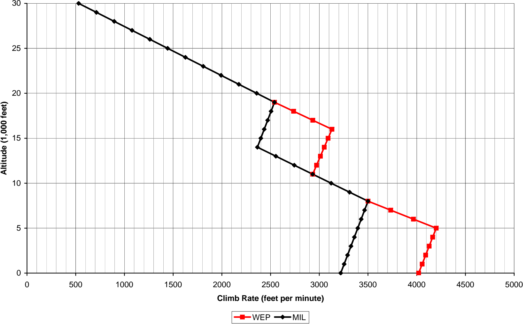
Aces High II Ki-84-IA Climb Rate
