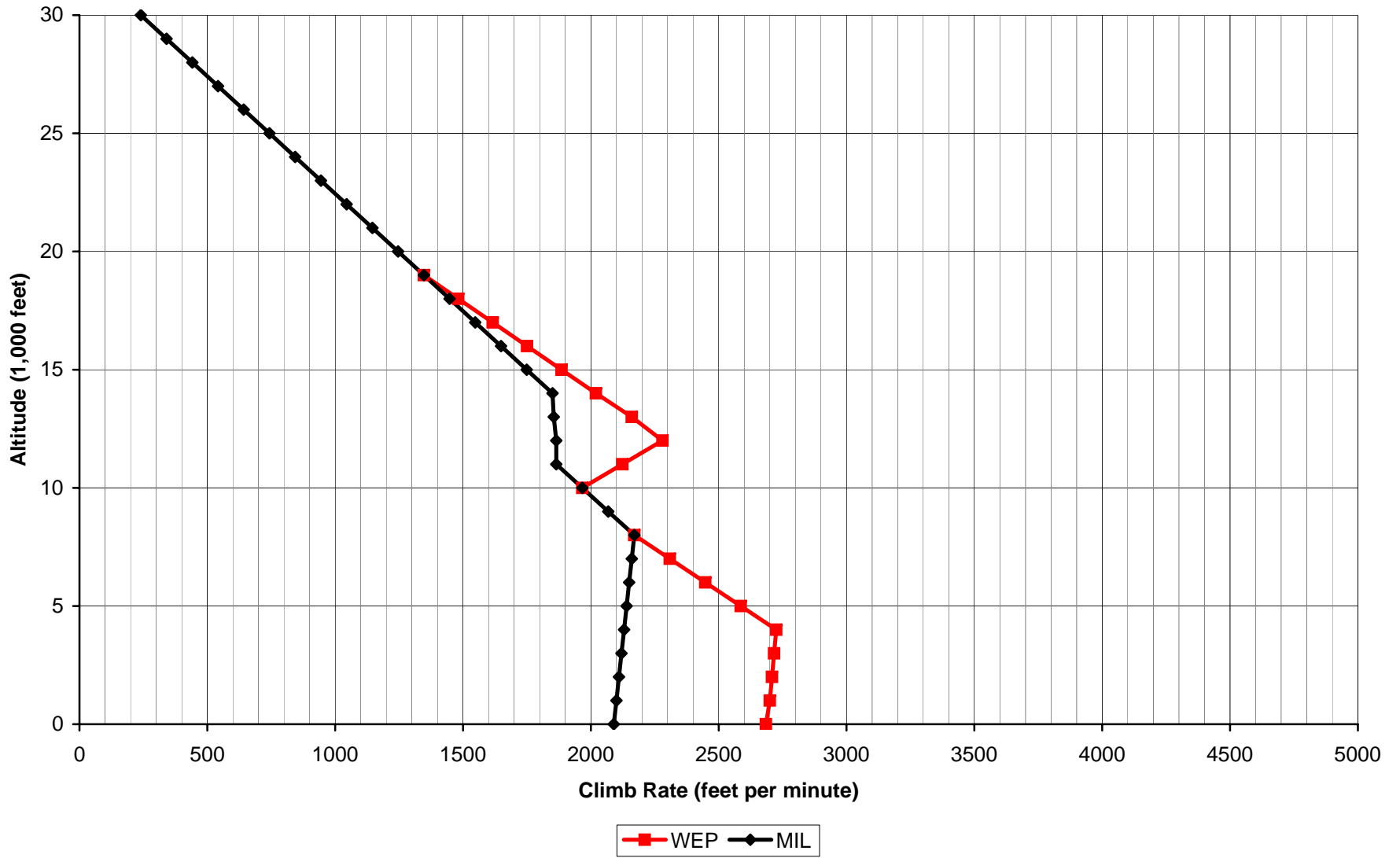
Aces High II Mosquito Mk VI Climb Rate
