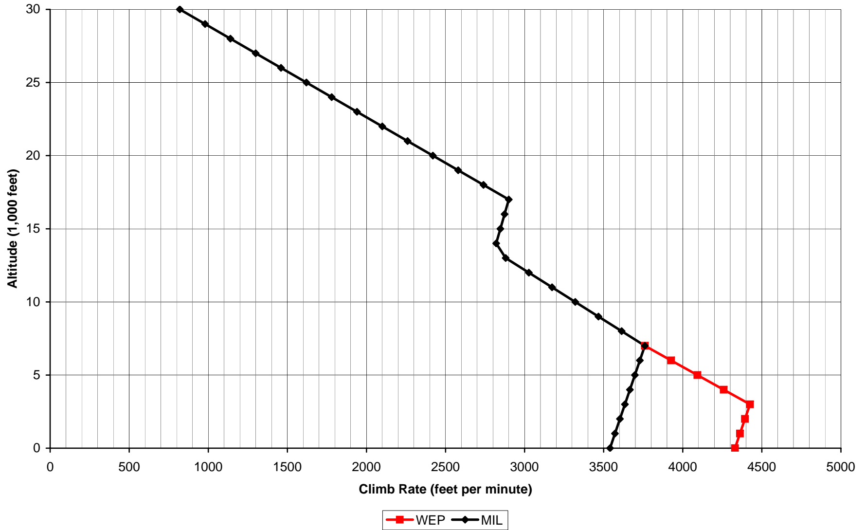
Aces High II La-5FN Climb Rate
