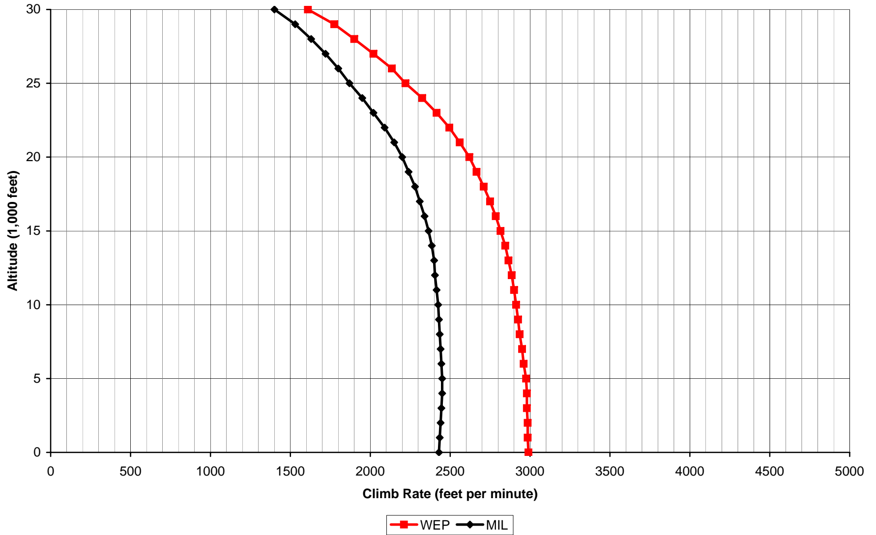
Aces High II P-47D-25 Climb Rate
