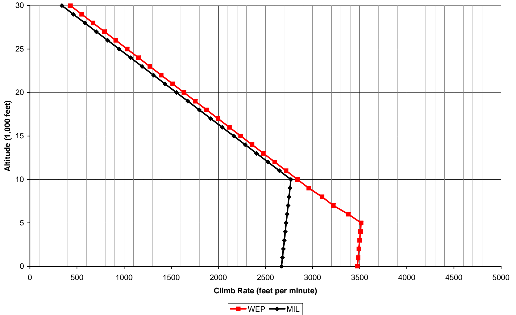
Aces High II Spitfire Mk I Climb Rate
