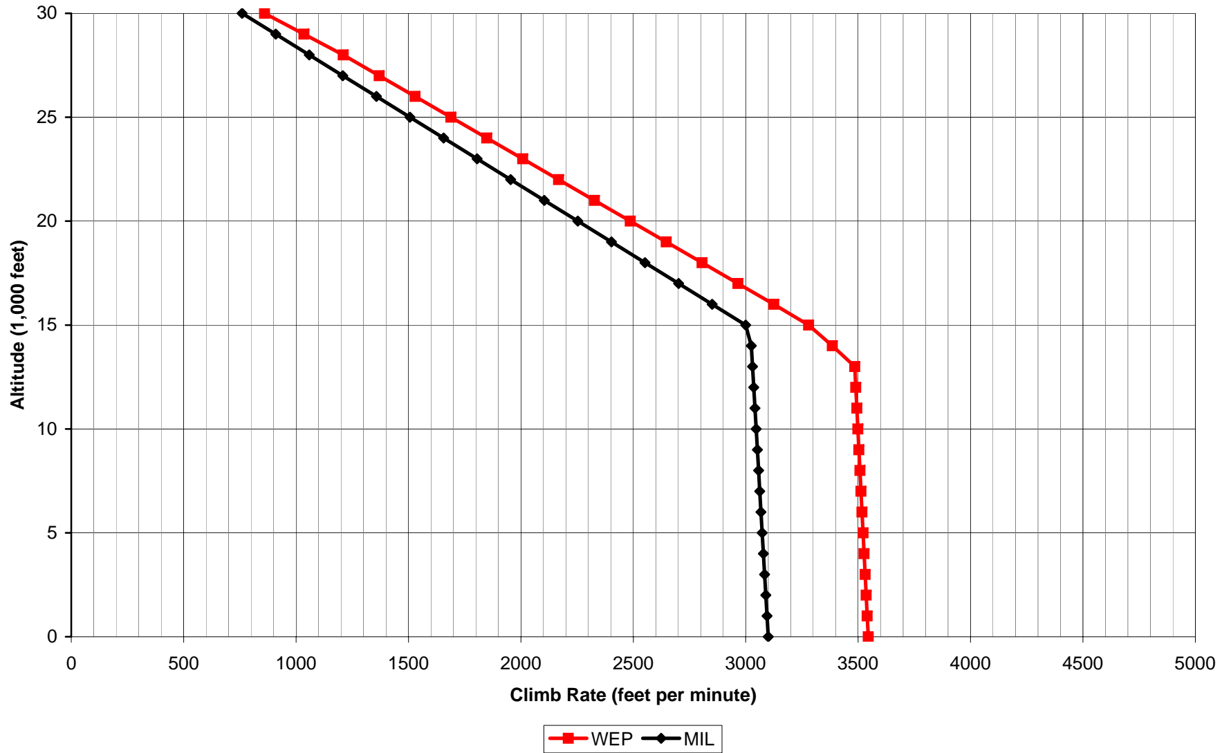
Aces High II C.202 Climb Rate
