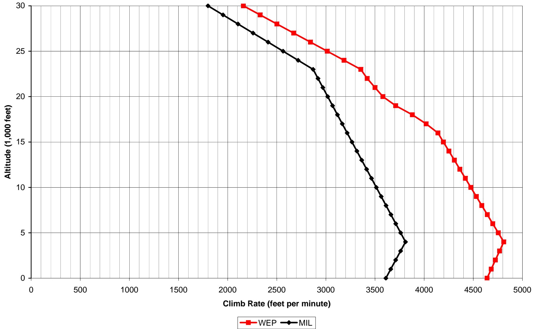
Aces High II Bf 109K-4 Climb Rate
