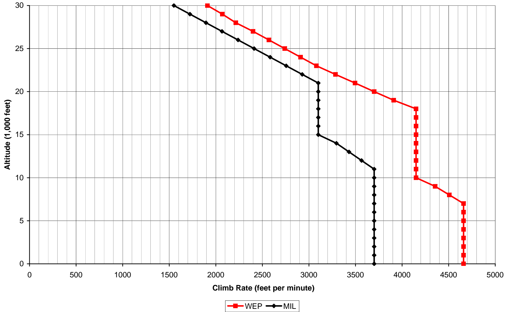
Aces High II Spitfire Mk XVI Climb Rate
