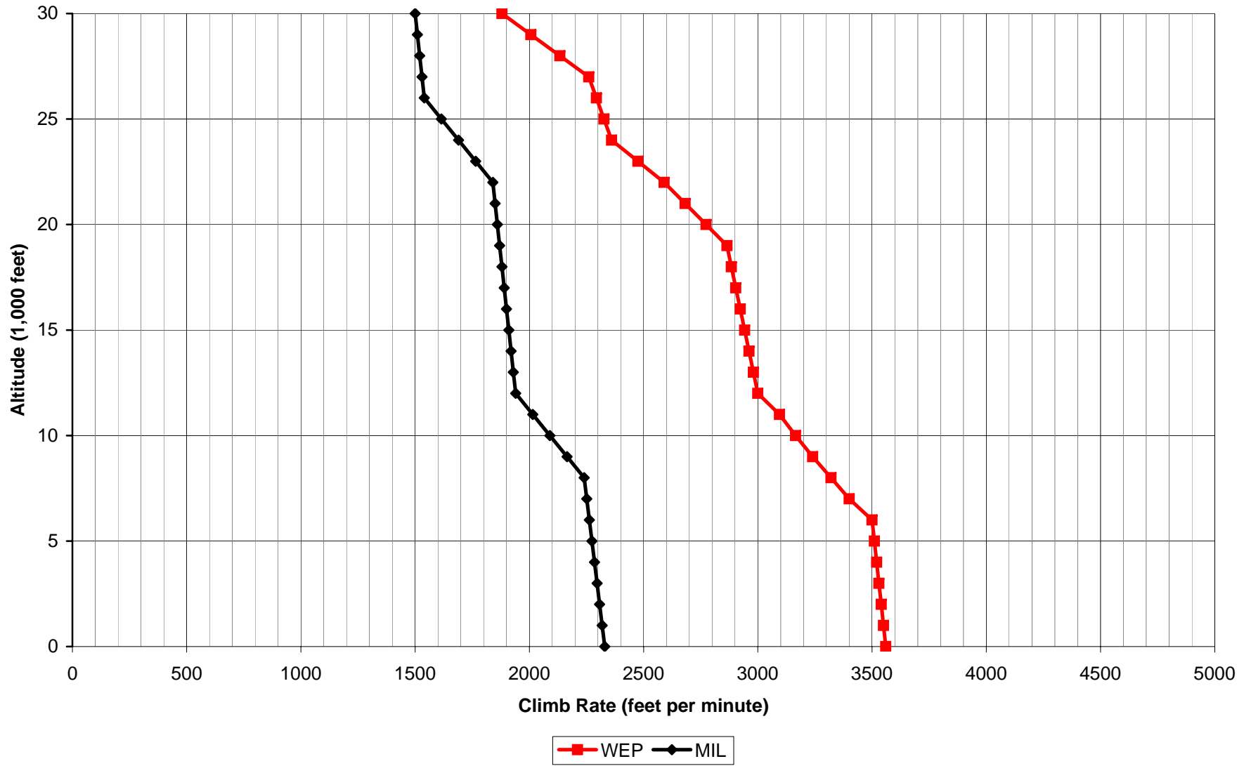
Aces High II Ta 152H-1 Climb Rate
