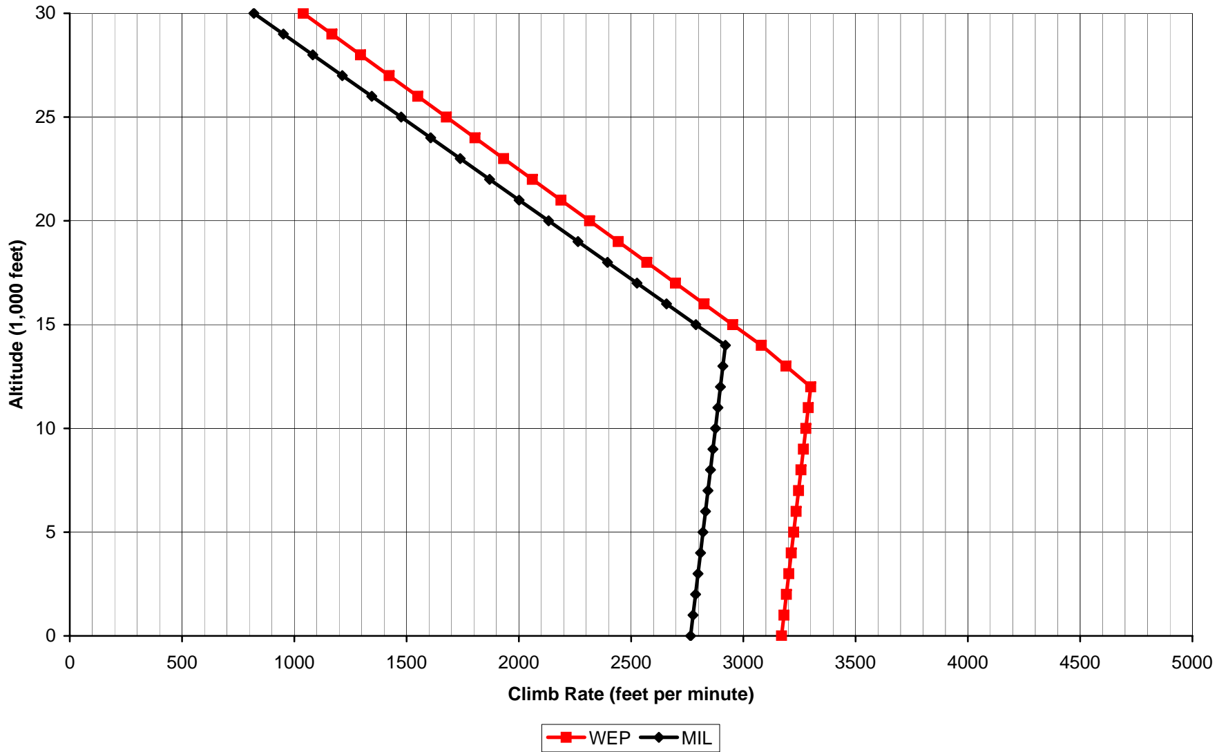
Aces High II Seafire Mk IIc Climb Rate
