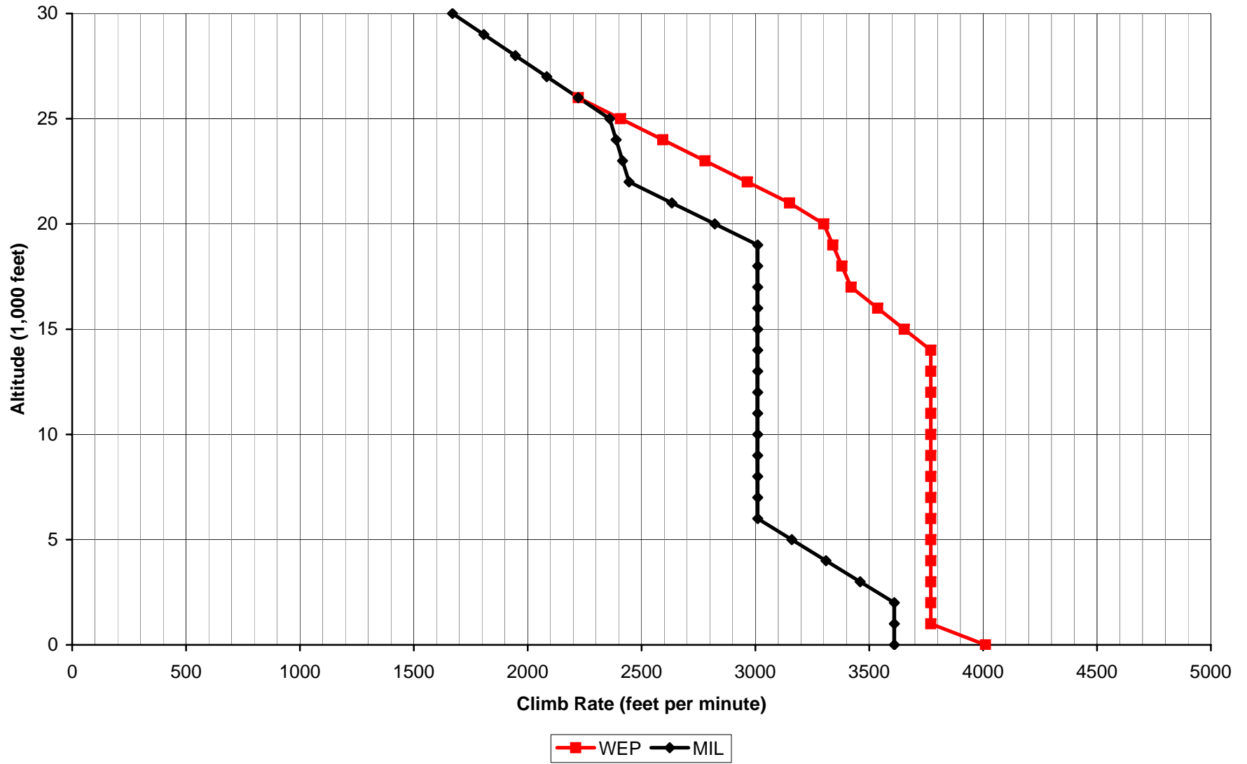
Aces High II F4U-4 Climb Rate
