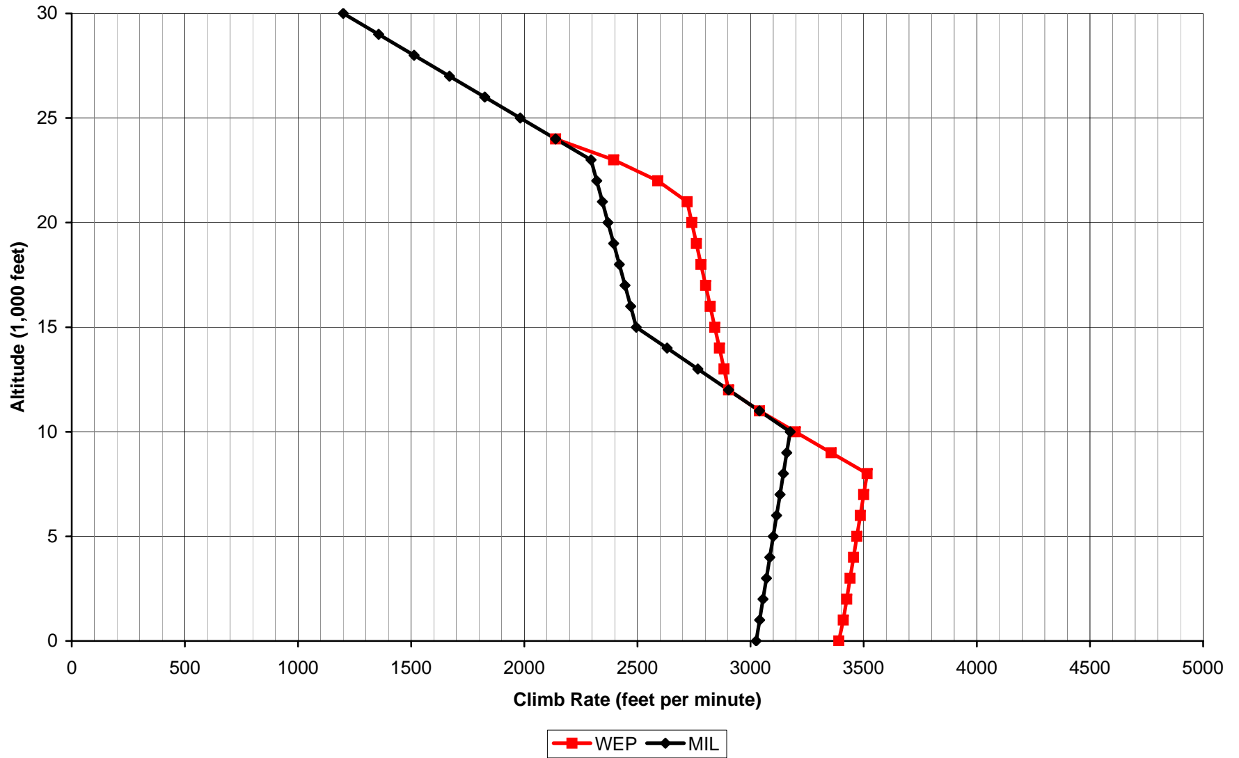
Aces High II P-51D Climb Rate
