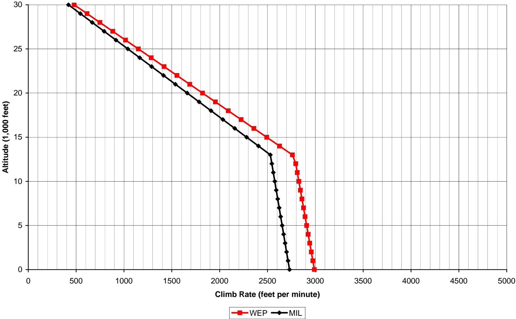
Aces High II Ki-61-I-TEI Climb Rate
