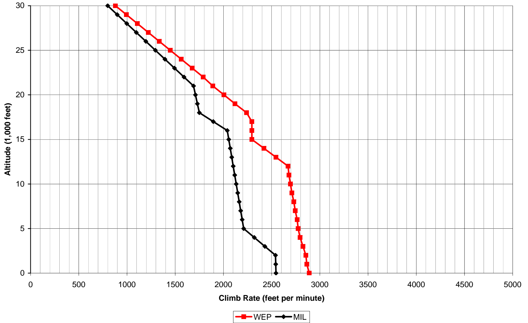
Aces High II F4U-1 Climb Rate
