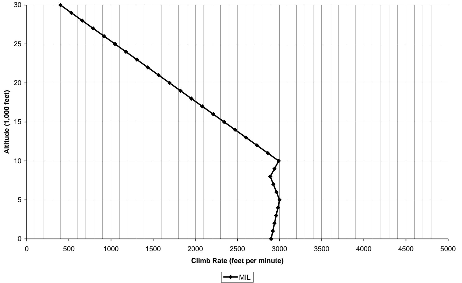
Aces High II Yak-9T Climb Rate
