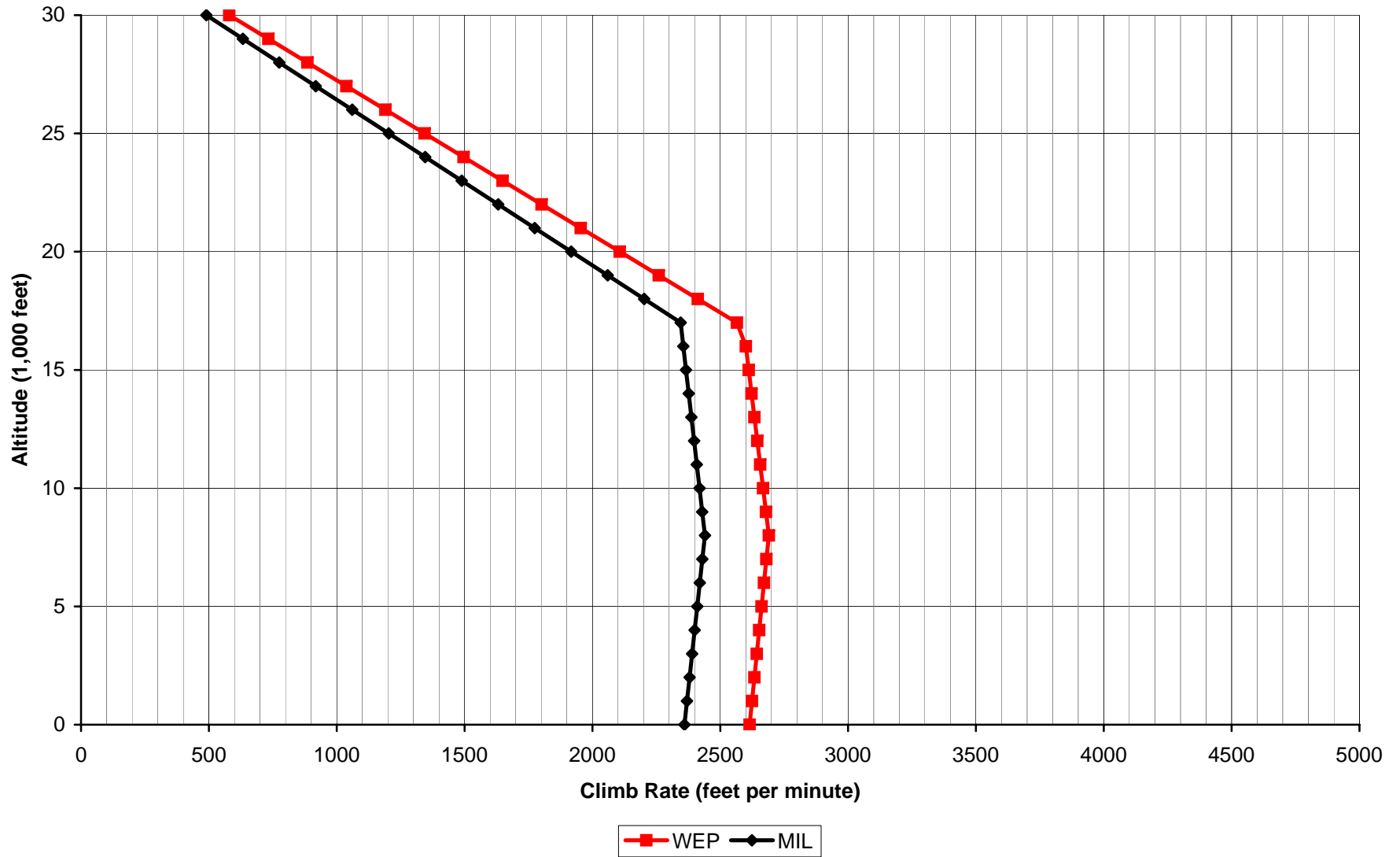
Aces High II Bf 110C-4B Climb Rate
