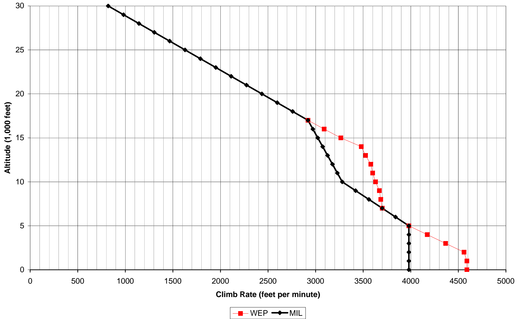
Aces High II Tempest Climb Rate
