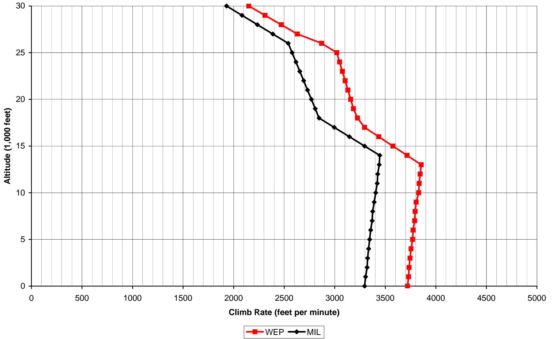
Aces High II Spitfire Mk IX Climb Rate
