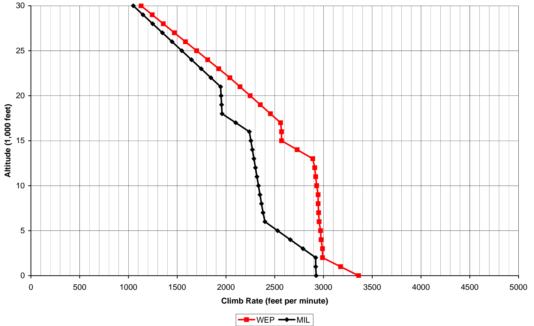
Aces High II F4U-1D Climb Rate
