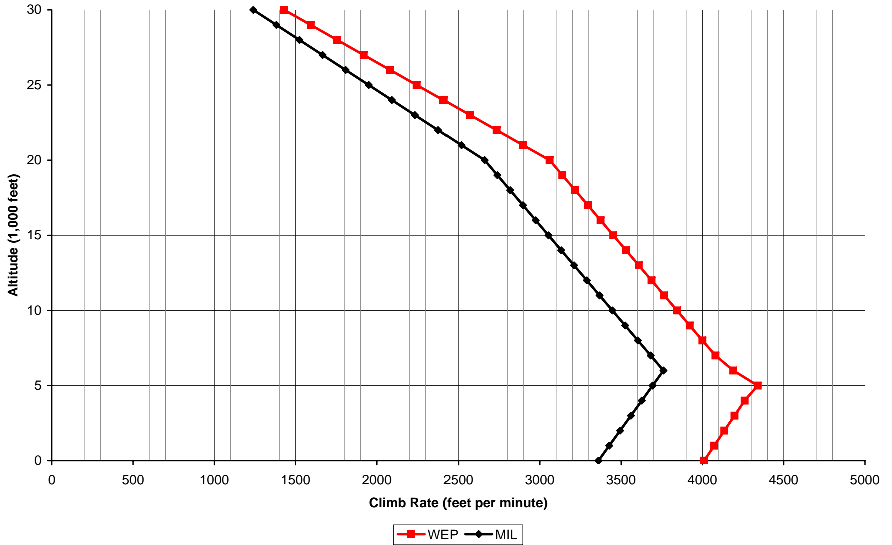
Aces High II Bf 109G-6 Climb Rate
