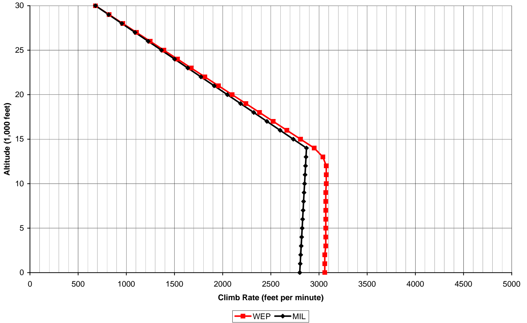
Aces High II Bf 109E-4 Climb Rate
